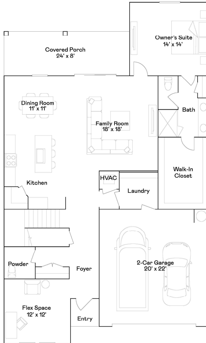
1st floor
